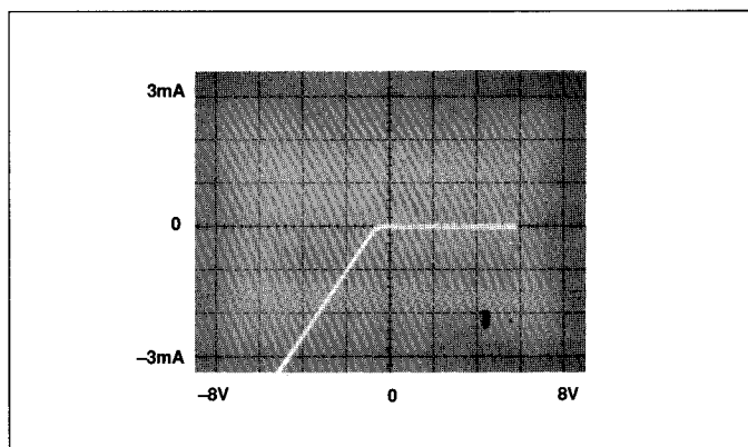
FIGURE 6: PM-7628 Digital Input Characteristic
