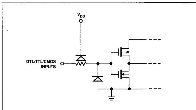
FIGURE 5: Digital Input Protection
