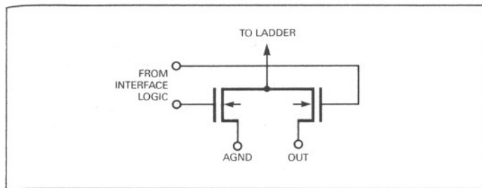
FIGURE 2: N-Channel Current Steering Switch
