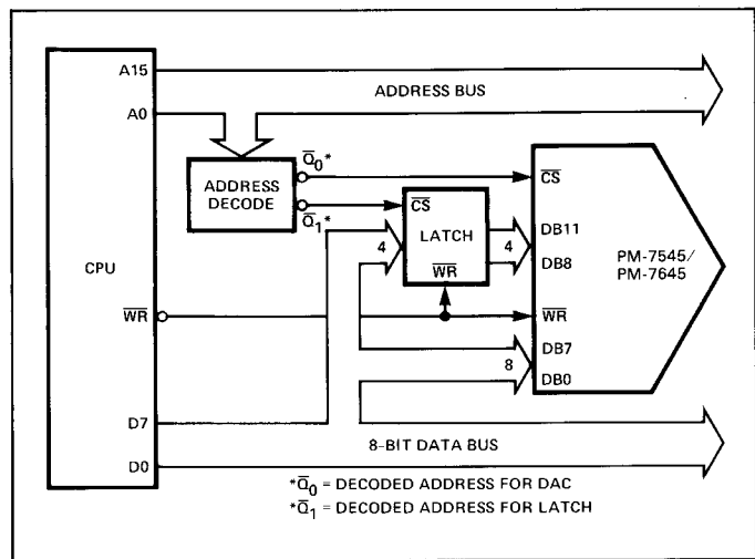
FIGURE 6: 8-Bit Processor to PM-7545/7645 Interface
