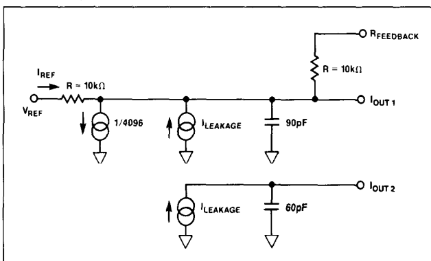
FIGURE 4: PM-7543 Equivalent Circuit (All Digital Inputs HIGH)
