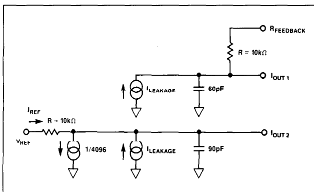
FIGURE 3: PM-7543 Equivalent Circuit (All Inputs LOW)
