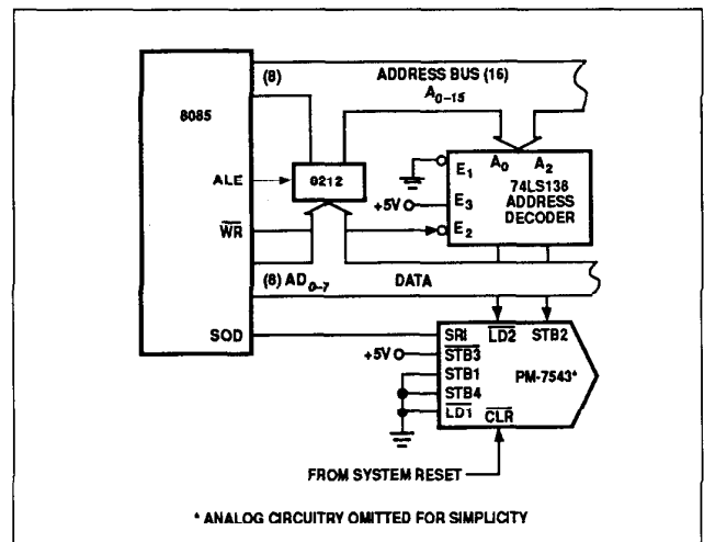
FIGURE 12: PM-7543 - 8085 Interface
