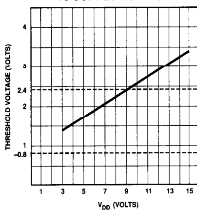
LOGIC THRESHOLD VOLTAGE vs SUPPLY VOLTAGE
