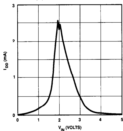
SUPPLY CURRENT vs LOGIC INPUT VOLTAGE
