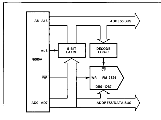
FIGURE 6: PM-7524/8085A Interface
