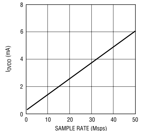
LTC2297: I_{OVD} vs Sample Rate, 5MHz Sine Wave Input, -1dB, O_{VDD} = 1.8\text{V}
