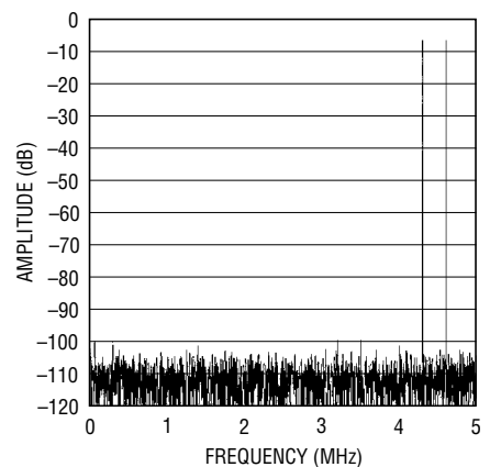
8192 Point 2-Tone FFT, f_{IN} = 4.3\text{MHz} and 4.6MHz, -1dB, 2V Range
