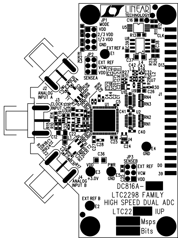
Silkscreen Top
