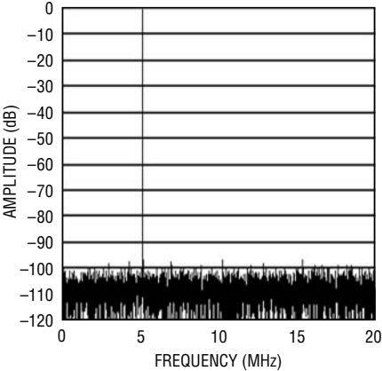
LTC2292: 8192 Point FFT, f_{IN} = 5\text{MHz} , -1dB, 2V Range, 40Msps
