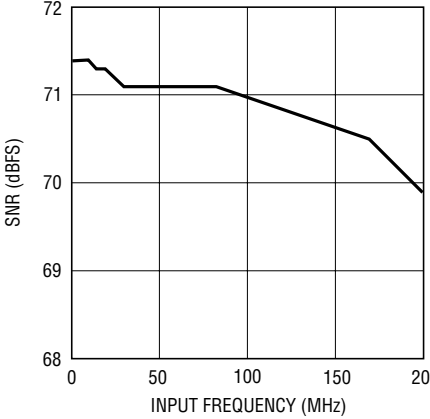
LTC2292: SNR vs Input Frequency, -1dB, 2V Range, 40Msps
