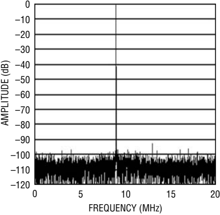
LTC2292: 8192 Point FFT, f_{IN} = 30\text{MHz} , -1dB, 2V Range, 40Msps
