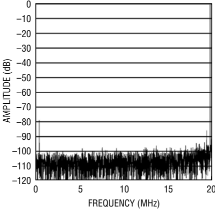
LTC2292: 8192 Point FFT, f_{IN} = 140\text{MHz} , -1dB, 2V Range, 40Msps
