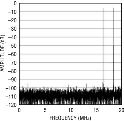
LTC2292: 8192 Point 2-Tone FFT, f_{IN} = 21.6\text{MHz} and 23.6\text{MHz} , -1dB, 2V Range, 40Msps
