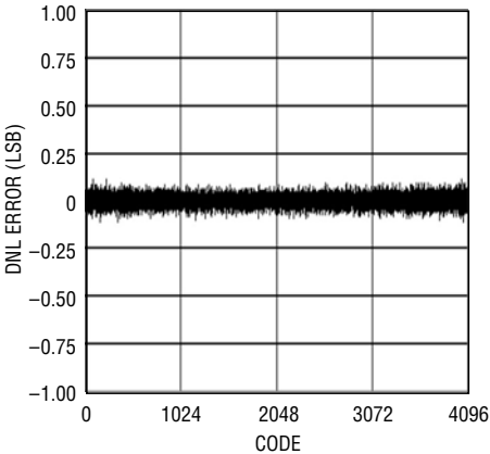
LTC2292: Typical DNL, 2V Range, 40Msps
