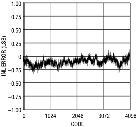
LTC2292: Typical INL, 2V Range, 40Msps
