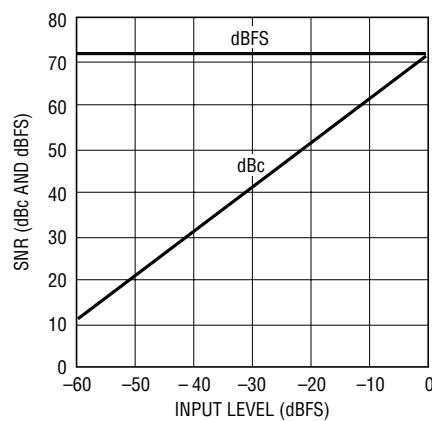
LTC2293: SNR vs Input Level, f_{IN} = 30\text{MHz} , 2V Range, 65Mps
