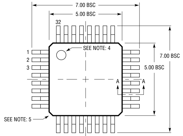
LU Package 32-Lead Plastic TQFP (5mm × 5mm) (Reference LTC DWG # 05-08-1735 Rev 0)
