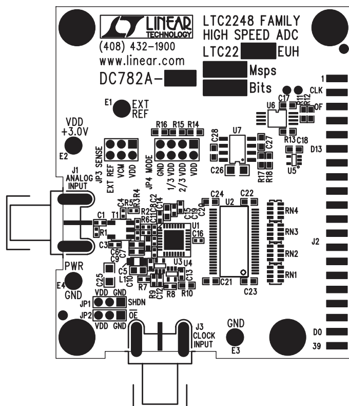
Silkscreen Top
