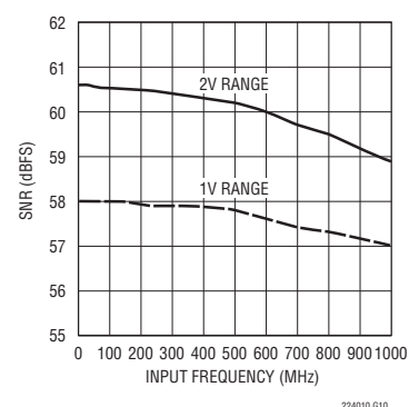
SNR vs Input Frequency
