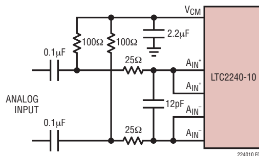
Figure 5. Capacitively-Coupled Drive
