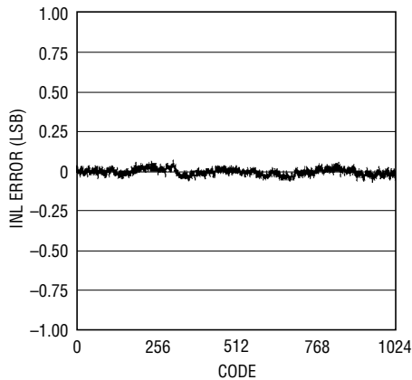
LTC2236: Typical INL, 2V Range, 25Msps
