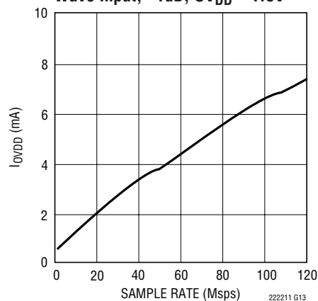
I_{OVDD} vs Sample Rate, 5MHz Sine Wave Input, -1\text{dB} , OV_{DD} = 1.8\text{V}
