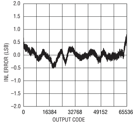
LTC2216 Integral Nonlinearity (INL) vs Output Code, Dither "On"
