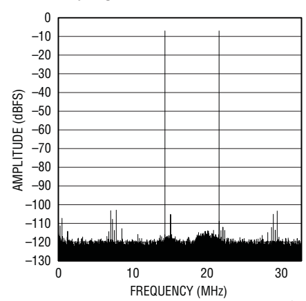
LTC2215 64k Point 2-Tone FFT, f_{IN} = 14.25\text{MHz} and 21.5\text{MHz} , -7\text{dBFS}
