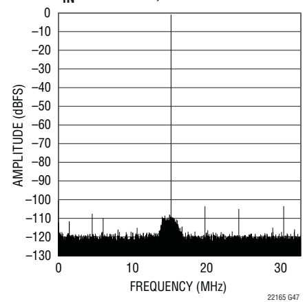
LTC2215 64k Point FFT, f_{IN} = 15.1\text{MHz} , -1\text{dBFS}
