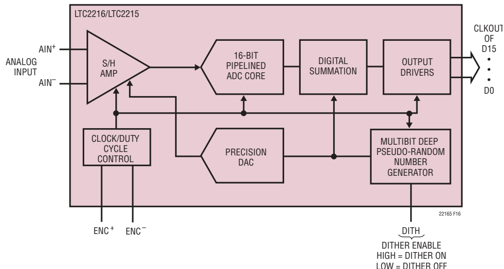
Figure 16. Functional Equivalent Block Diagram of Internal Dither Circuit
