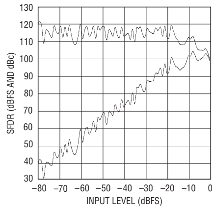
LTC2204: SFDR vs Input Level, f_{IN} = 15.1\text{MHz} , \text{DITH} = 1 , \text{RAND} = 1
