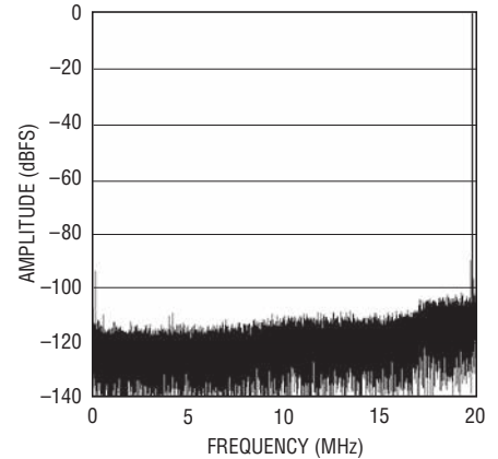
LTC2204: 64K Point FFT, 40Msps, f_{IN} = 140.1\text{MHz} , -1\text{dBFS} , PGA = 0, DITH = 0
