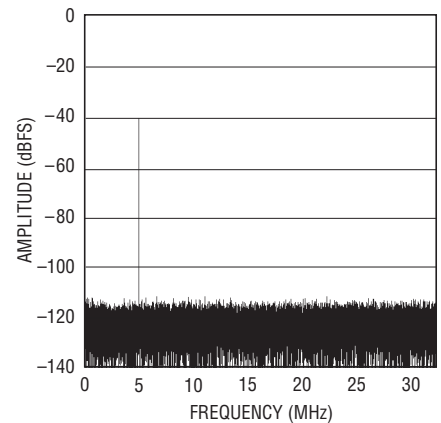
LTC2205: 64K Point FFT, f_{IN} = 5.1\text{MHz} , -40dBFS, PGA = 0, DITH = 1
