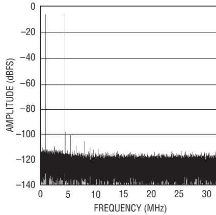
LTC2205: 64K Point FFT, f_{IN1} = 64.1\text{MHz} , -7\text{dBFS} , f_{IN2} = 20.1\text{MHz} , -7\text{dBFS} , \text{PGA} = 0
