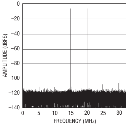
LTC2205: 64K Point FFT, f_{IN1} = 14.9\text{MHz} , -7\text{dBFS} , f_{IN2} = 20.1\text{MHz} , -7\text{dBFS} , \text{PGA} = 0
