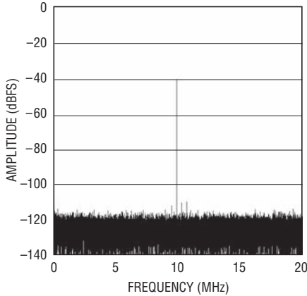
LTC2204: 64K Point FFT, 40Msps, f_{IN} = 70.1\text{MHz} , -40\text{dBFS} , PGA = 0, DITH = 0
