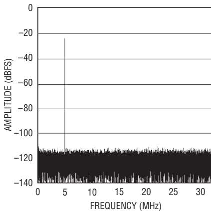
LTC2205: 64K Point FFT, f_{IN} = 5.1\text{MHz} , -25dBFS, PGA = 0, DITH = 1
