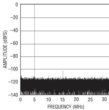
LTC2205: 64K Point FFT, 65Msps, f_{IN} = 5.1\text{MHz} , -1dBFS, PGA = 1, DITH = 0
