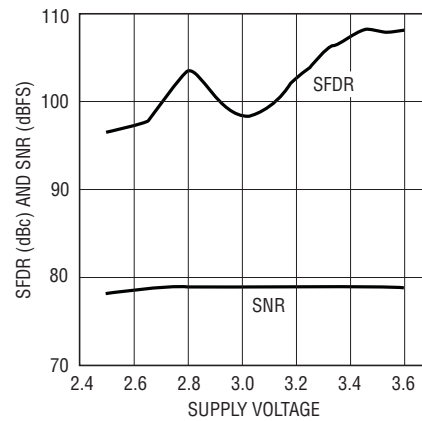
LTC2205: SFDR and SNR vs Supply Voltage, f_{IN} = 5.1\text{MHz} , 65MSPS, PGA = 0
