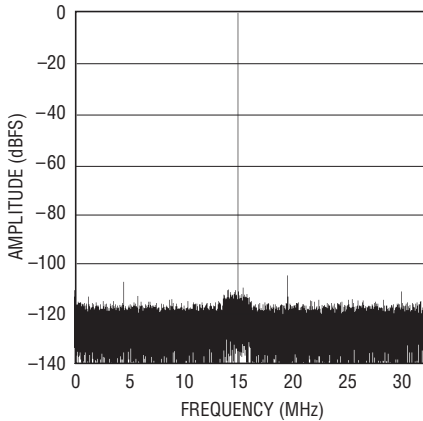
LTC2205: 64K Point FFT, 65Msps, f_{IN} = 15.1\text{MHz} , -25\text{dBFS} , PGA = 0, DITH = 1
