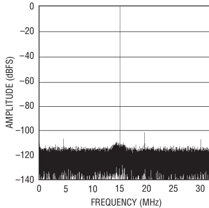
LTC2205: 64K Point FFT, 65Msps, f_{IN} = 15.1\text{MHz} , -40\text{dBFS} , PGA = 0, DITH = 0
