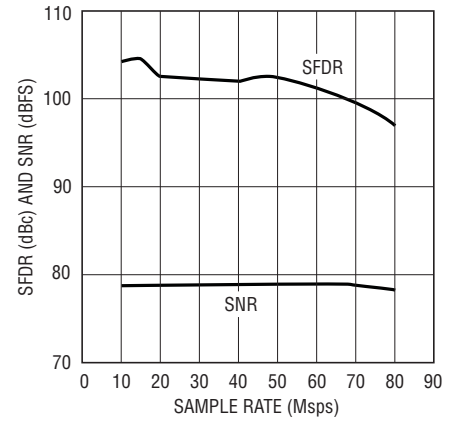
LTC2204: SFDR and SNR vs Sample Rate, f_{IN} = 5.1\text{MHz} , -1\text{dBFS} , PGA = 0, DITH = 0, RAND = 0
