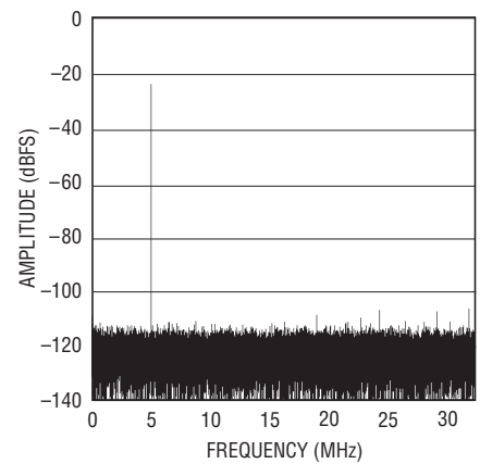
LTC2205: 64K Point FFT, f_{IN} = 5.1\text{MHz} , -25dBFS, PGA = 0, DITH = 0
