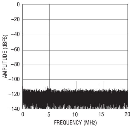
LTC2204: 64K Point FFT, 40Msps, f_{IN} = 5.1\text{MHz} , -25dBFS, PGA = 1, DITH = 0
