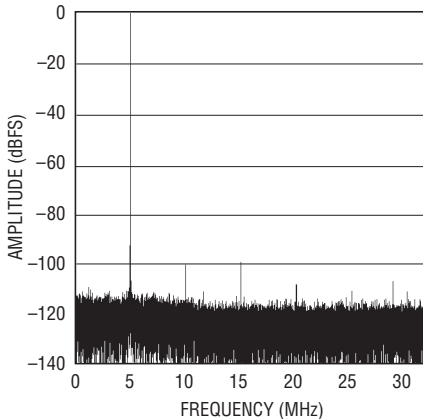
LTC2205: 64K Point FFT, 65Msps, f_{IN} = 70.1\text{MHz} , -1\text{dBFS} , PGA = 0, DITH = 0
