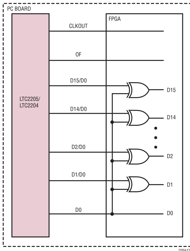
Figure 13. Descrambling a Scrambled Digital Output
