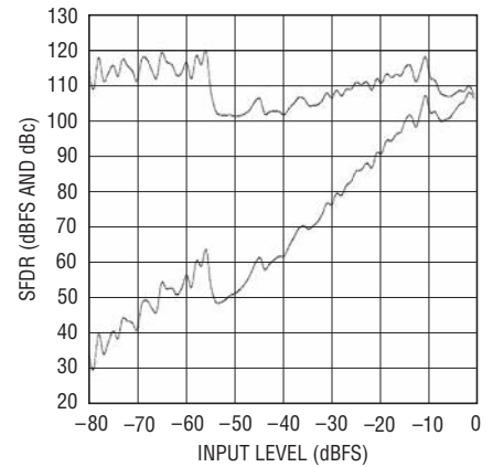
LTC2205: SFDR vs Input Level, f_{IN} = 5.1\text{MHz} , \text{DITH} = 0 , \text{RAND} = 1 , \text{PGA} = 0
