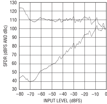
LTC2204: SFDR vs Input Level, f_{IN} = 5.1\text{MHz} , \text{DITH} = 0 , \text{RAND} = 1
