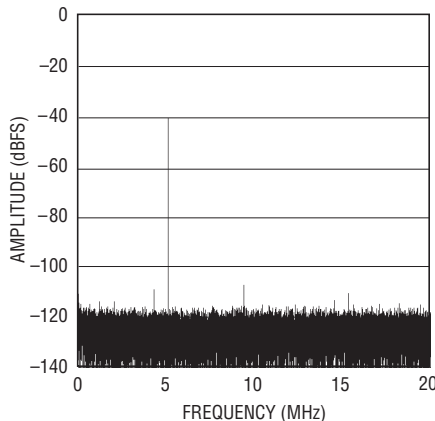
LTC2204: 64K Point FFT, 40Msps, f_{IN} = 5.1\text{MHz} , -40dBFS, PGA = 0, DITH = 0
