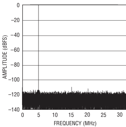
LTC2205: 64K Point FFT, f_{IN} = 5.1\text{MHz} , -1dBFS, PGA = 0, DITH = 0
