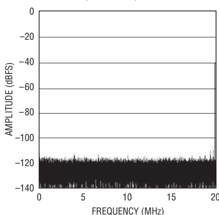
LTC2204: 64K Point FFT, 40Msps, f_{IN} = 140.1\text{MHz} , -25\text{dBFS} , PGA = 0, DITH = 0
