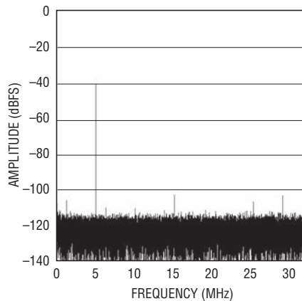
LTC2205: 64K Point FFT, f_{IN} = 5.1\text{MHz} , -40dBFS, PGA = 0, DITH = 0
