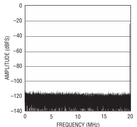
LTC2204: 64K Point FFT, 40Msps, f_{IN} = 140.1\text{MHz} , -25\text{dBFS} , PGA = 0, DITH = 1
