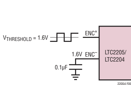
Figure 9. Single-Ended ENC Drive, Not Recommended for Low Jitter
