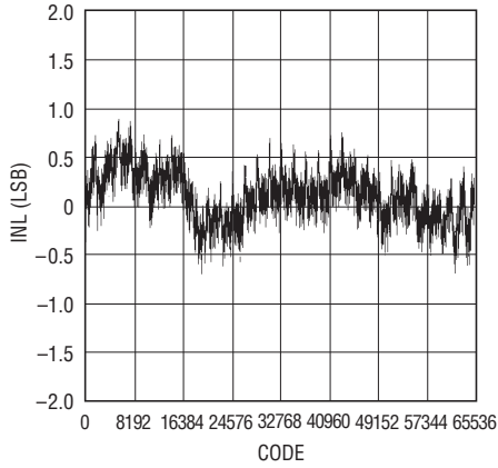
LTC2205: INL (Integral Non-Linearity) vs Code
