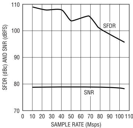
LTC2205: SFDR and SNR vs Sample Rate, f_{IN} = 5.1\text{MHz} , -1dBFS, PGA = 0
