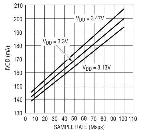
LTC2205: IVDD vs Sample Rate, f_{IN} = 5.1\text{MHz} , -1dBFS
