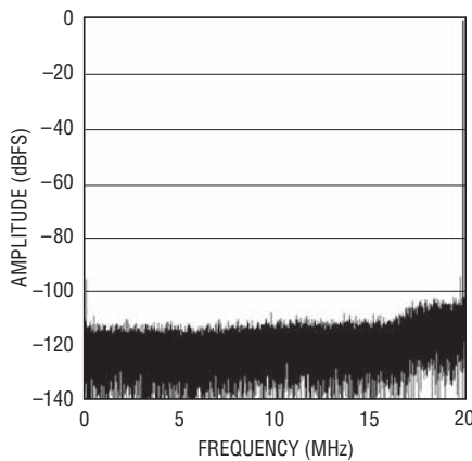
LTC2204: 64K Point FFT, 40Msps, f_{IN} = 140.1\text{MHz} , -1\text{dBFS} , PGA = 1, DITH = 0
