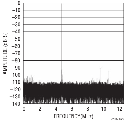
LTC2203: 32K Point FFT, f_{IN} = 70.1\text{MHz} , -1\text{dBFS} , \text{PGA} = 1
