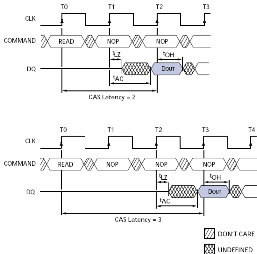
Figure 22. SDRAM CAS Timing
