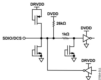
Figure 11. Equivalent SDIO/DCS or SMI SDFS Circuit
