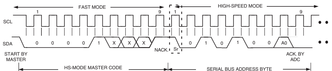
Figure 28. Placing the Part into High Speed Mode
