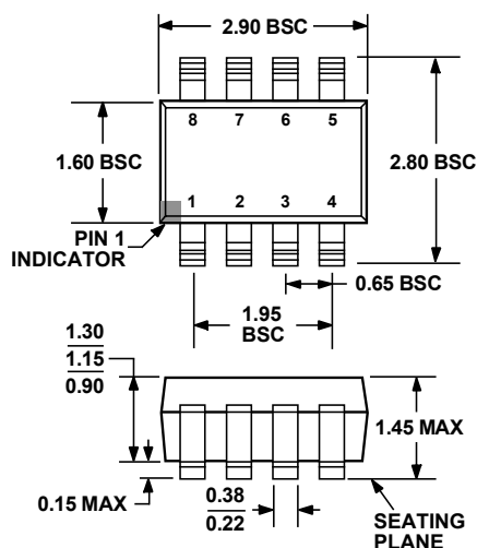
Figure 30. .8-Lead Small Outline Transistor Package (SOT-23) (RJ-8) Dimensions shown in millimeters
