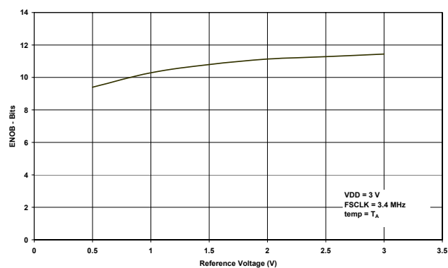
Figure 8 ENOB vs Reference Voltage, VDD = 3V
