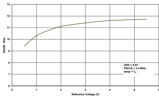
Figure 7 ENOB vs Reference Voltage, VDD = 5.5V
