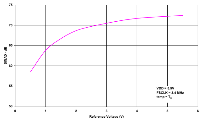
Figure 9 SINAD vs Reference Voltage, VDD = 5.5V
