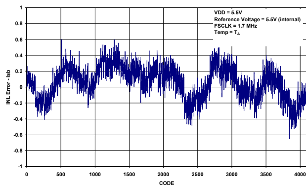
Figure 13 INL VDD = 5.5
