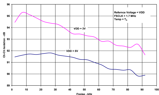
Figure 17 Channel-to-Channel Isolation
