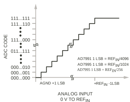
Figure 22 . AD7991/AD7995/AD7999 Transfer Characteristic
