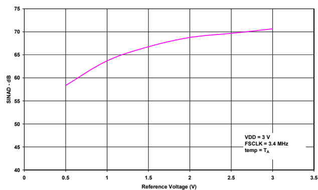
Figure 10. SINAD vs Reference Voltage, VDD = 3V
