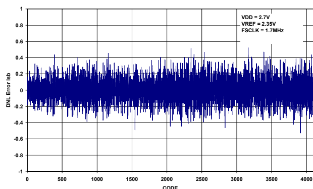
Figure 5 DNL error, VDD = 2.7V, Reference Voltage = 2.35V
