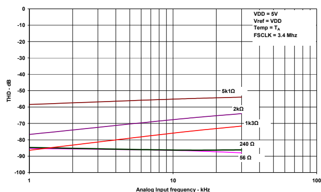
Figure 25. THD vs Analog Input Frequency for various source Impedances for VDD = 5V
