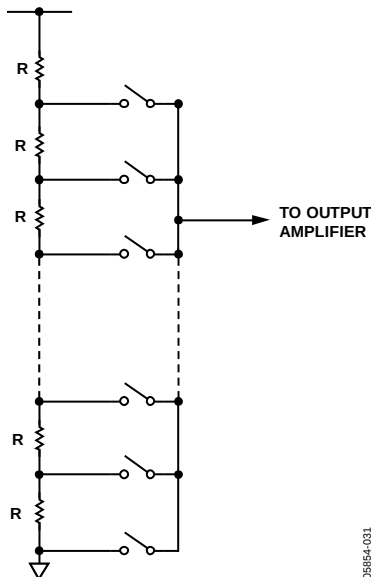
Figure 24. Resistor String
