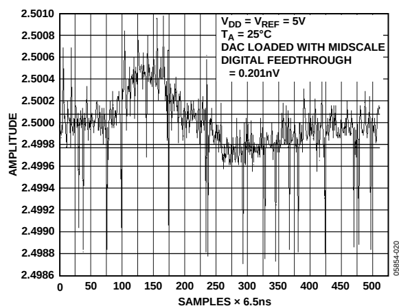
Figure 18. Digital Feedthrough
