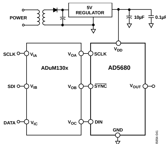
Figure 37. AD5680 with a Galvanically Isolated Interface
