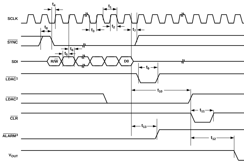
Figure 3. Write Timing Diagram
