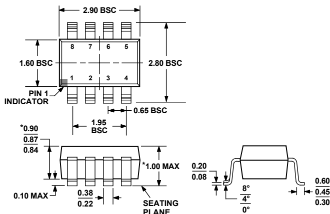
Figure 65. 8-Lead Thin Small Outline Transistor Package [TSOT] (UJ-8)
