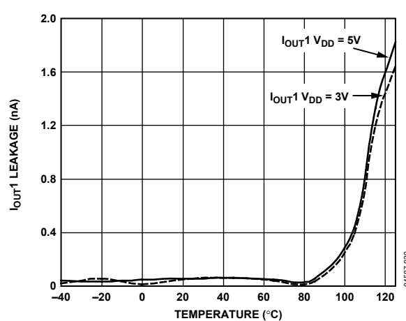
Figure 22. I_{\text{OUT1}} Leakage Current vs. Temperature
