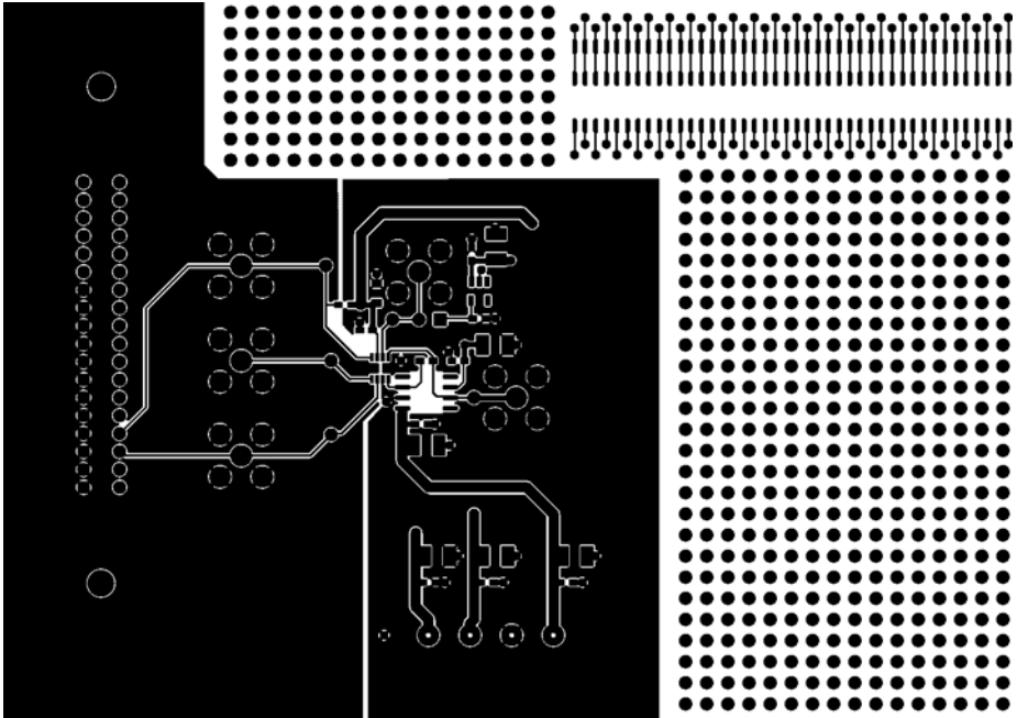
Figure 62. Component-Side Artwork
