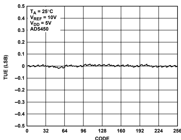
Figure 15. TUE vs. Code (8-Bit DAC)
