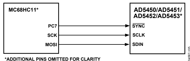
Figure 58. MC68HC11-to-AD5450/AD5451/AD5452/AD5453 Interface
