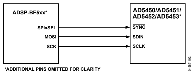
Figure 55. ADSP-BF5xx-to-AD5450/AD5451/AD5452/AD5453 Interface
