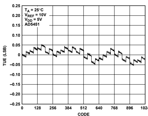
Figure 16. TUE vs. Code (10-Bit DAC)
