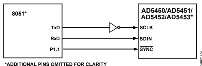
Figure 57. 80C51/80L51-to-AD5450/AD5451/AD5452/AD5453 Interface
