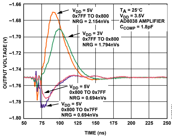
Figure 31. Midscale Transition, V_{REF} = 3.5 V
