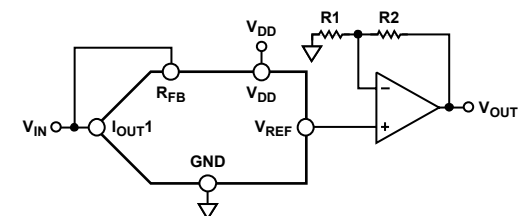
Figure 45. Single-Supply Voltage-Switching Mode
