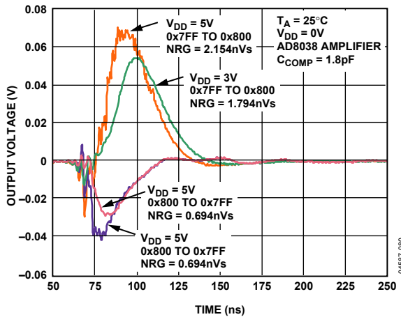
Figure 30. Midscale Transition, V_{REF} = 0 V
