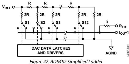
Figure 42. AD5452 Simplified Ladder
