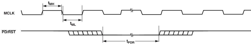
Figure 1. MCLK and \overline{\text{RESET}} Timing
