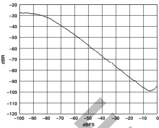
Figure 20. THD + N Ratio vs. Input Amplitude, Input 1 kHz, SR 48 kHz, 24-Bit
