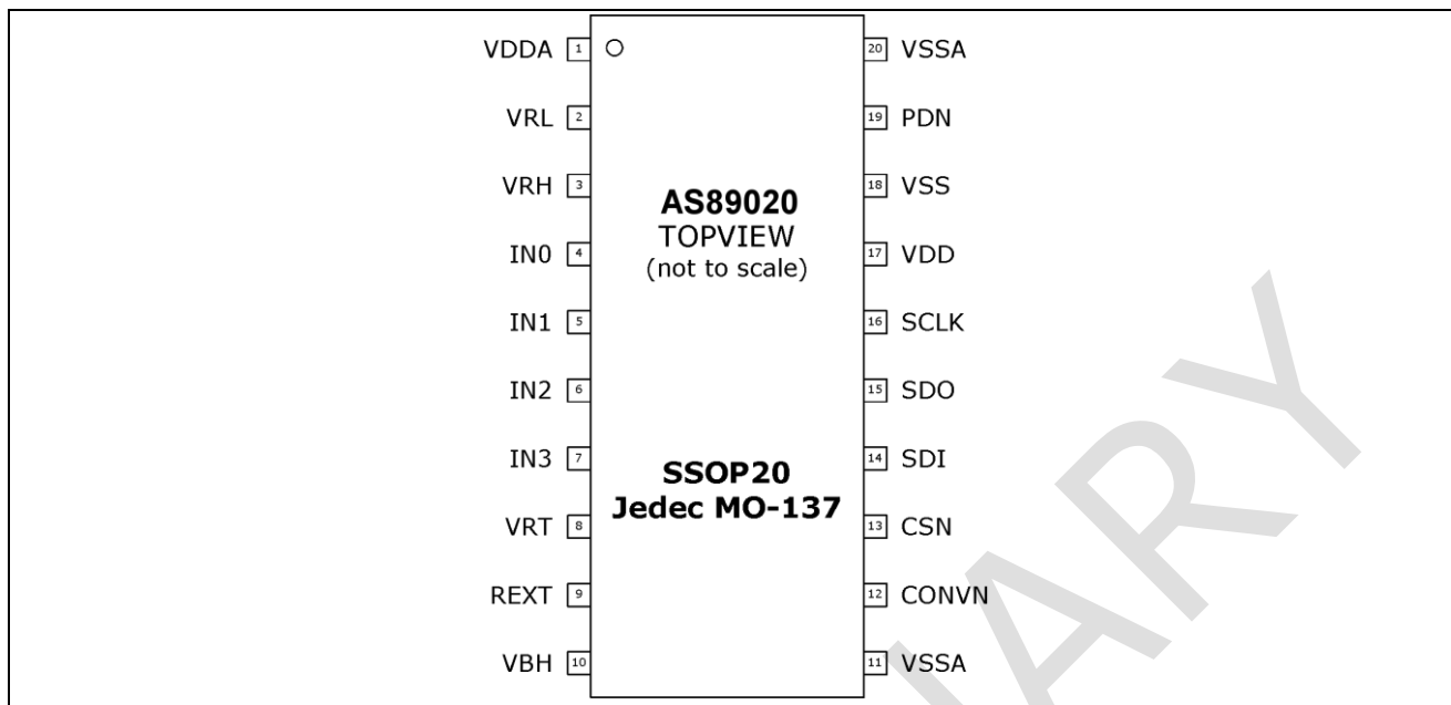
Figure 12: Pin Configuration
