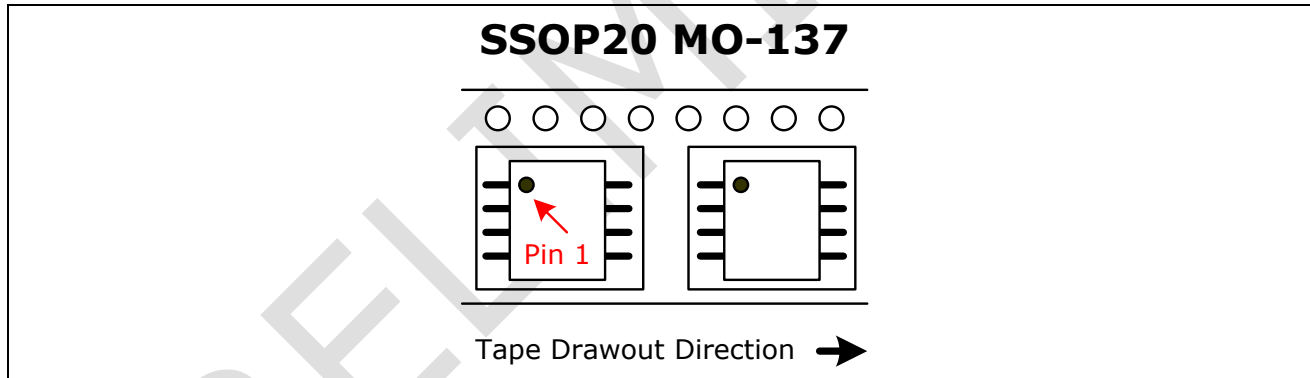
Figure 13: Standard packing
