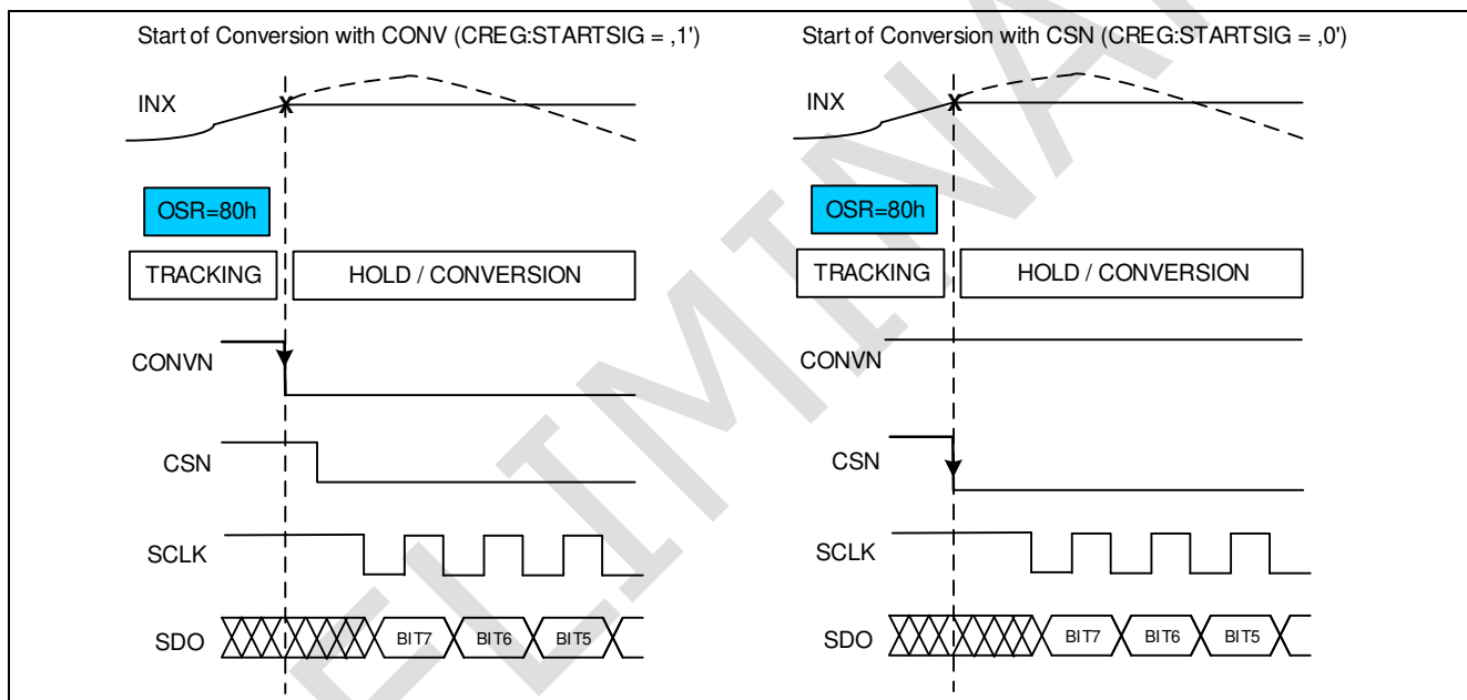
Figure 5: start of conversion with CONV or CSN
