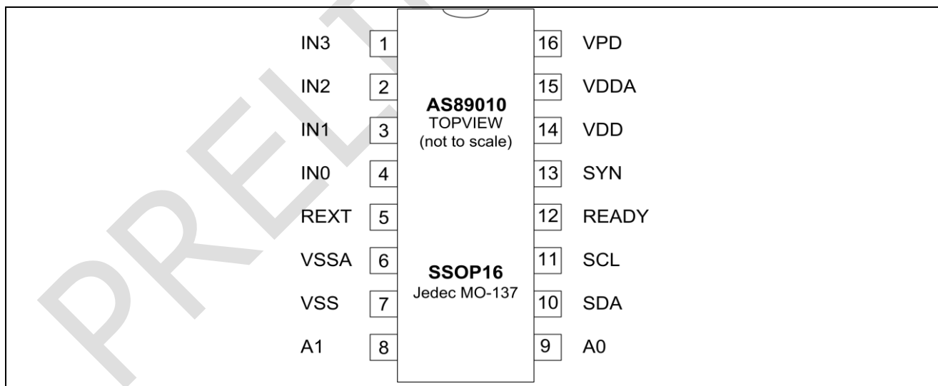
Figure 16: Pin configuration
