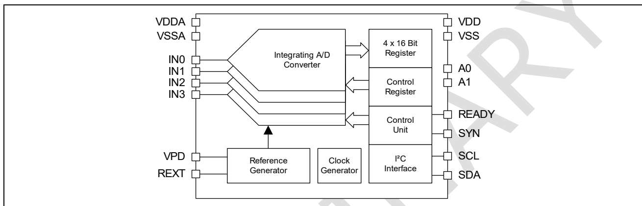
Figure 2: Block diagram
