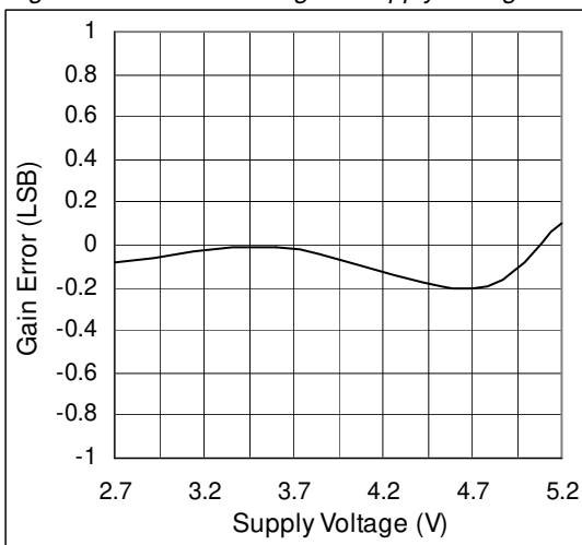
Figure 15. Gain Matching vs. Supply Voltage
