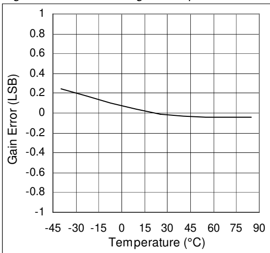
Figure 13. Gain Matching vs. Temperature
