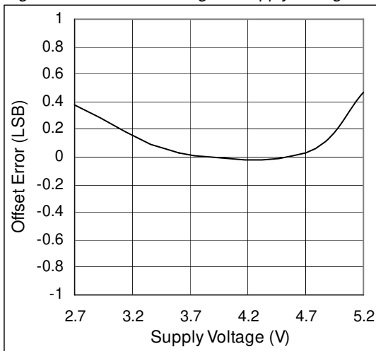
Figure 11. Offset Matching vs. Supply Voltage
