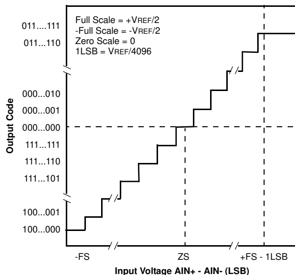
Figure 27. Two's Complement Transfer Function for RANGE = 0 and MODE = 0
