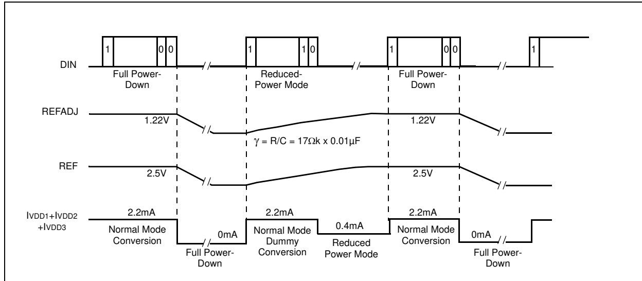
Figure 30. Full Power-Down Timing Waveforms (AS1531)
