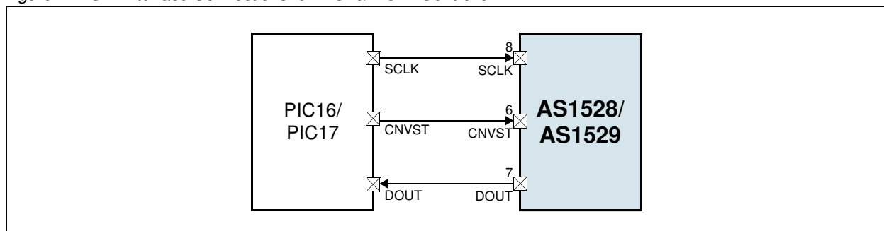
Figure 27. SPI Interface Connections for PIC16/PIC17 Controller
