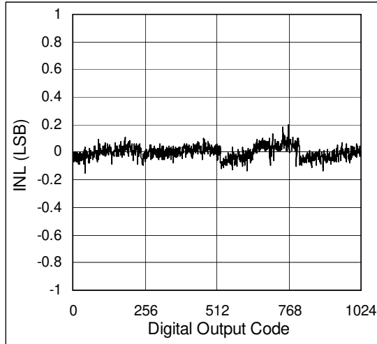
Figure 5. Integral Nonlinearity vs. Digital Output Code
