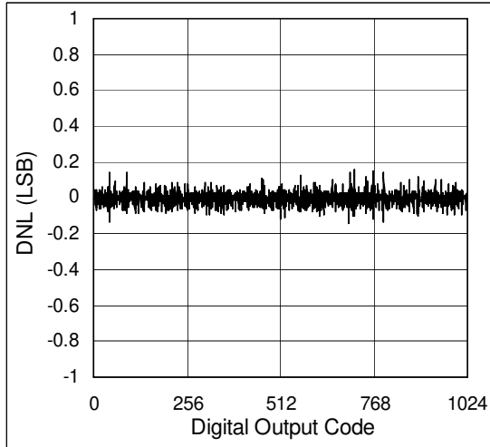
Figure 6. Differential Nonlinearity vs. Digital Output Code
