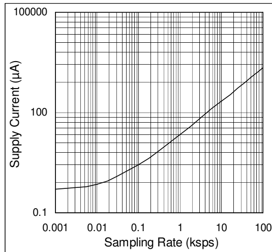
Figure 31. Average Supply Current vs. Sampling Rate (AS1523, FULLPD, and External Reference)
