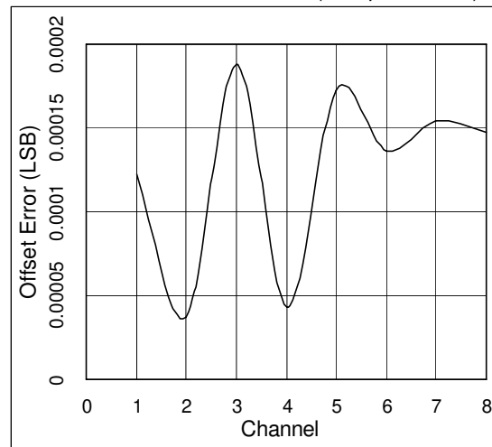
Figure 8. Offset Error vs. Channel; V_{DD} = 2.7V , T = 25^{\circ}C , all DACs (except selected) = 0x00h
