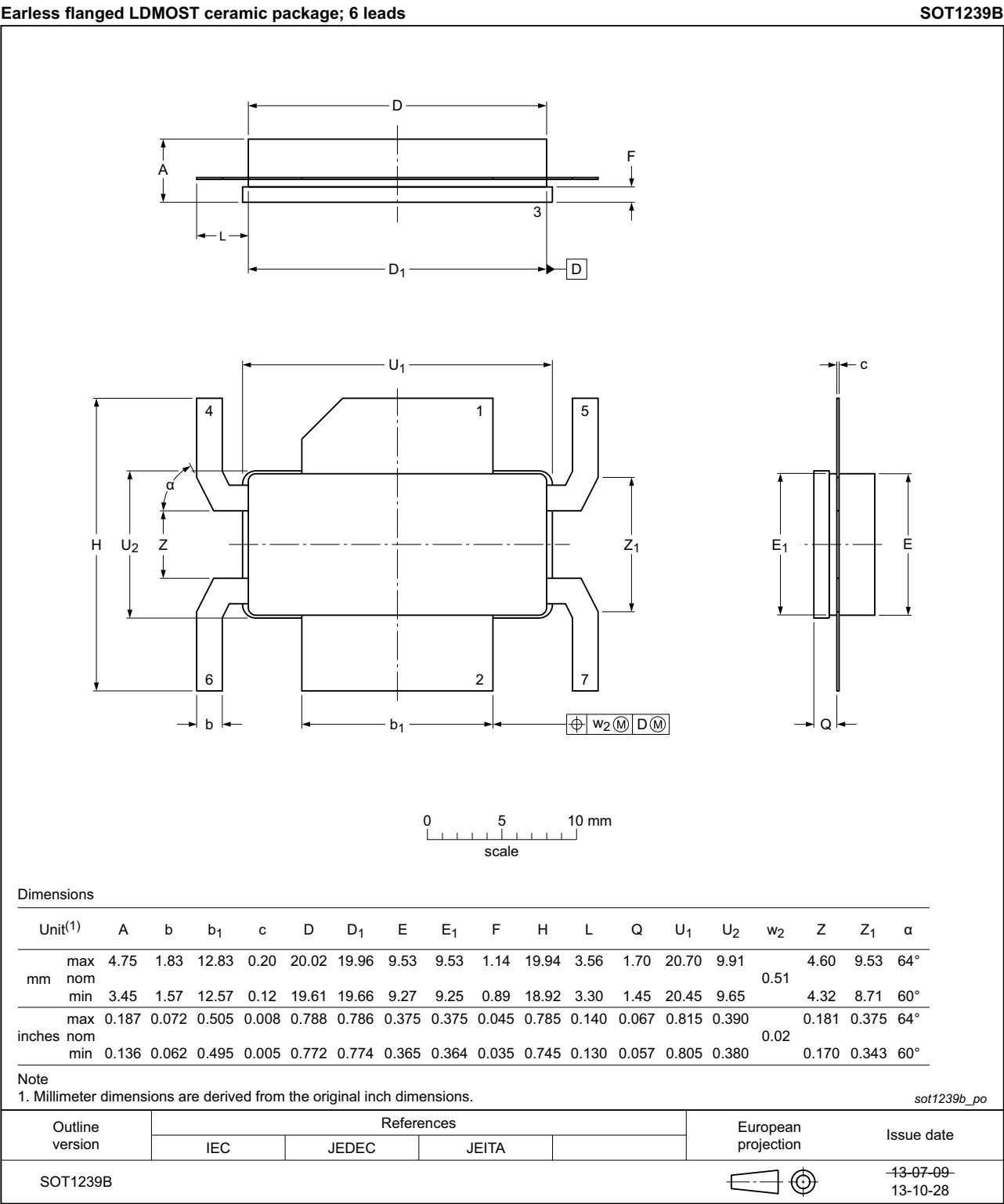
Fig 9. Package outline SOT1239B
