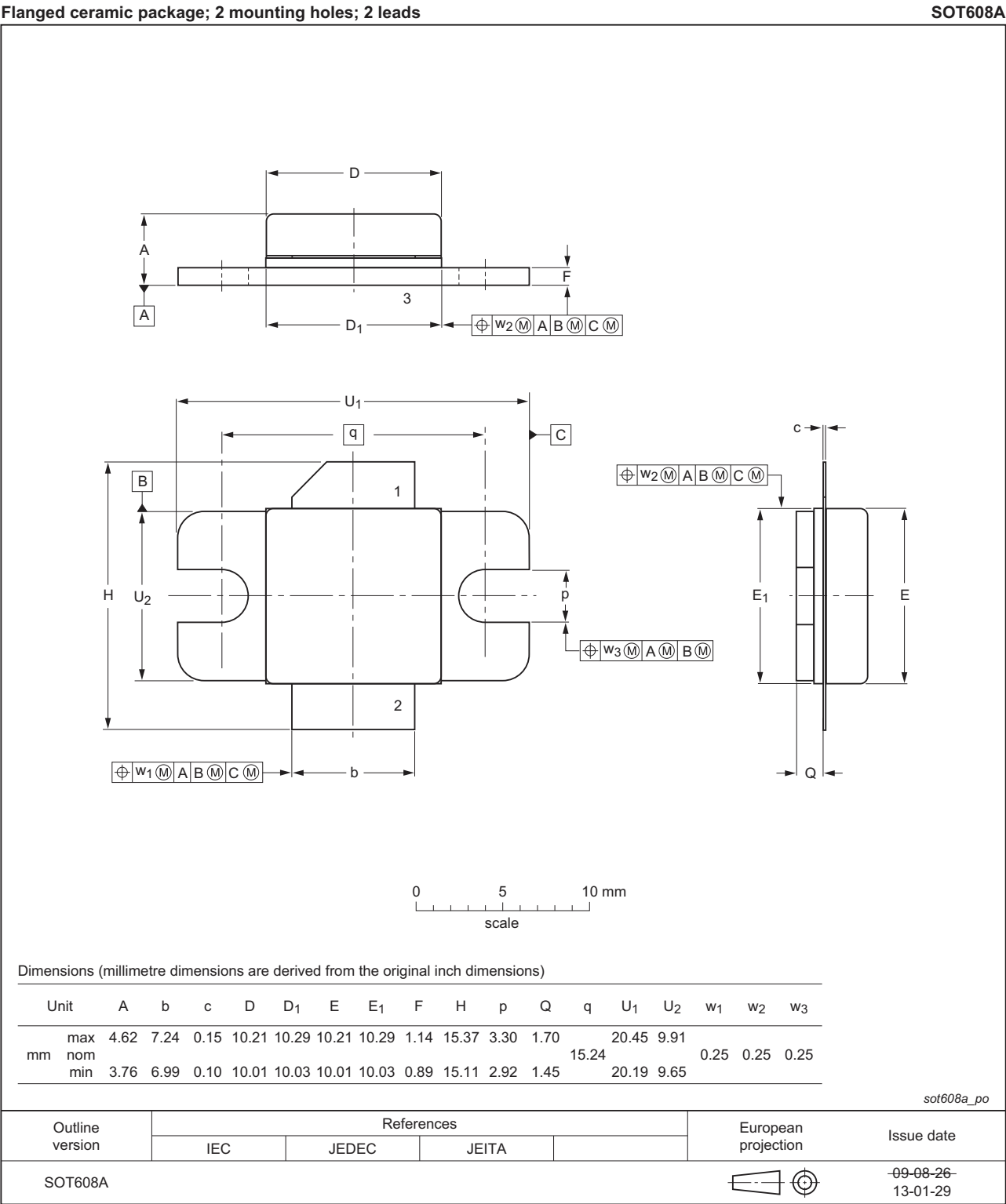
Fig 14. Package outline SOT608A
