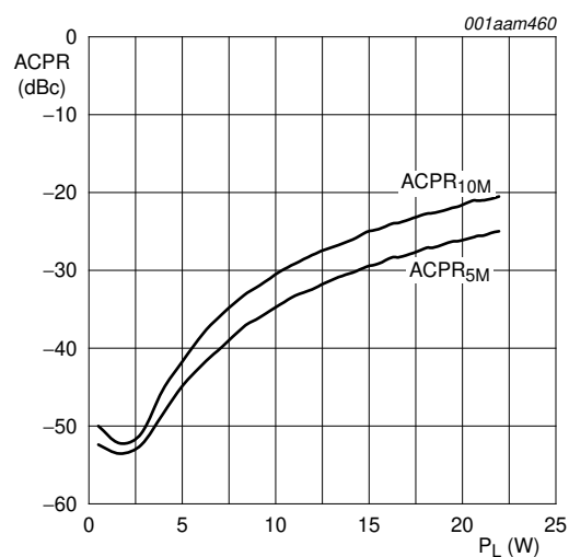
Fig 4. ACPR at 5 MHz and at 10 MHz as function of load power; typical values
