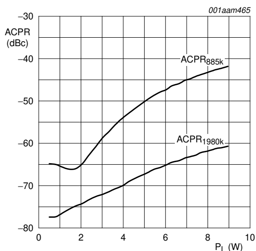
Fig 9. ACPR at 885 kHz and at 1980 kHz as function of load power; typical values
