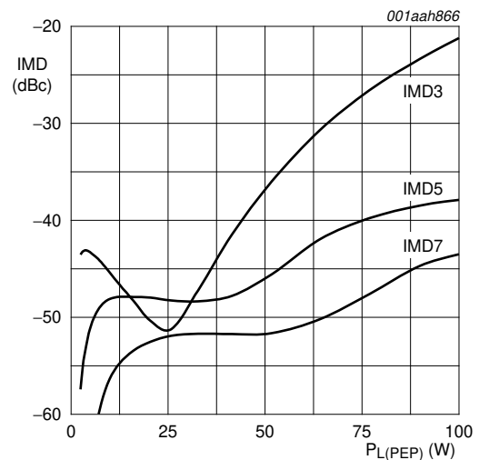
Fig 3. Two-tone CW intermodulation distortion as a function of peak envelope load power; typical values
