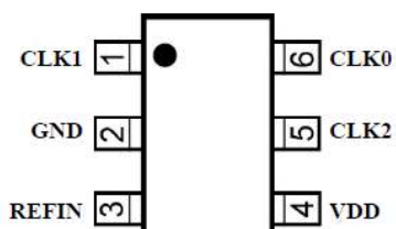
SOT23-6L package
