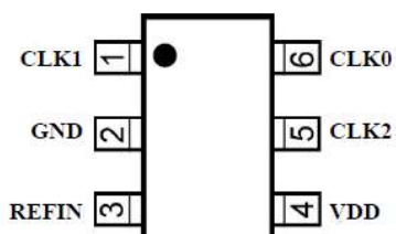
SOT23-6L package
